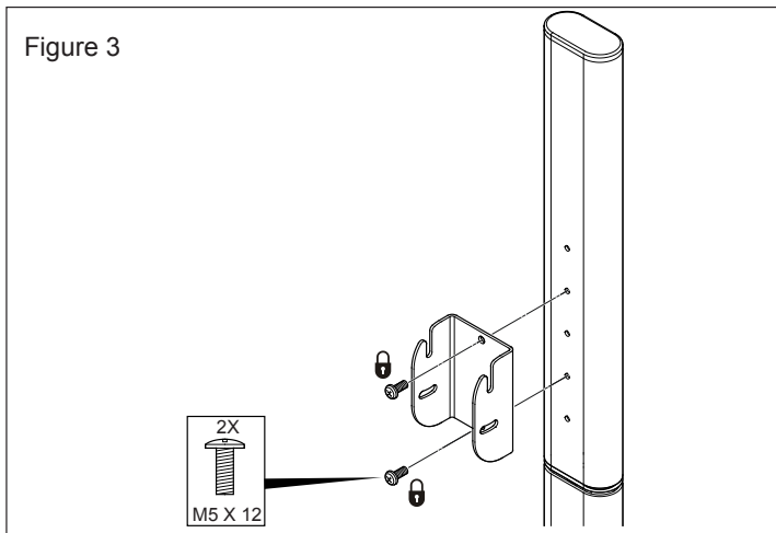
Attach bracket to Ascent with 2 M5 X 12 screws as shown in Figure 3.
